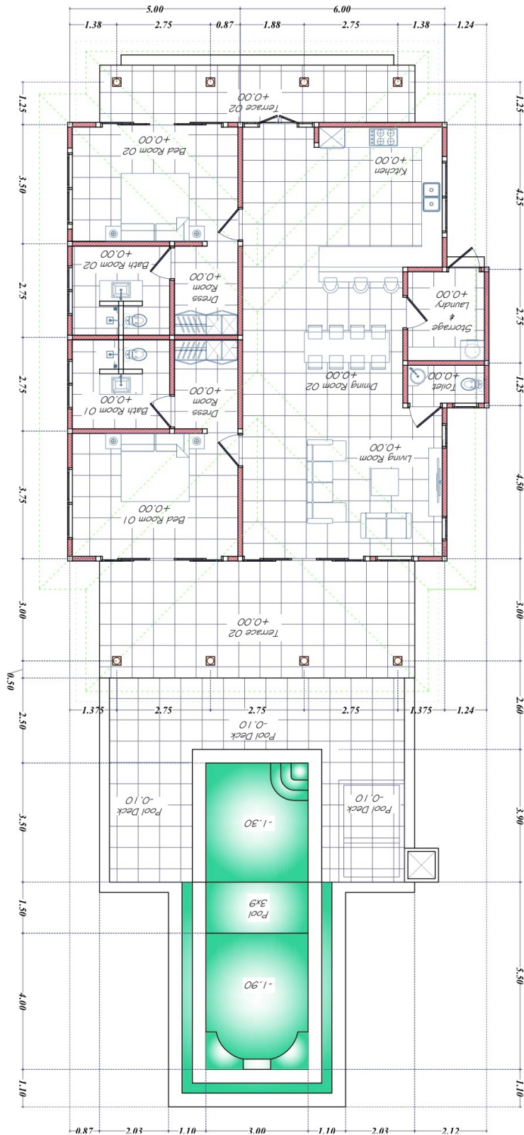
Main House Plan Skala 1:100
